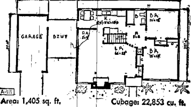
Area: 1,405 sq. ft. Cubage: 22,853 cu. ft.
